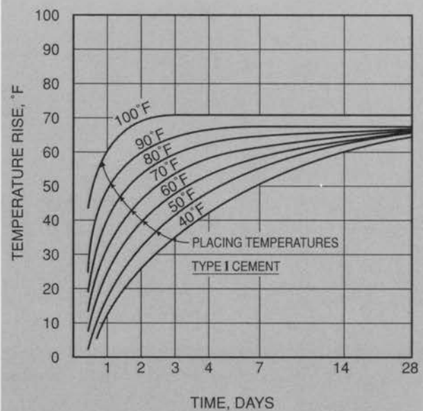
Temperature Rise of Mass Concrete
