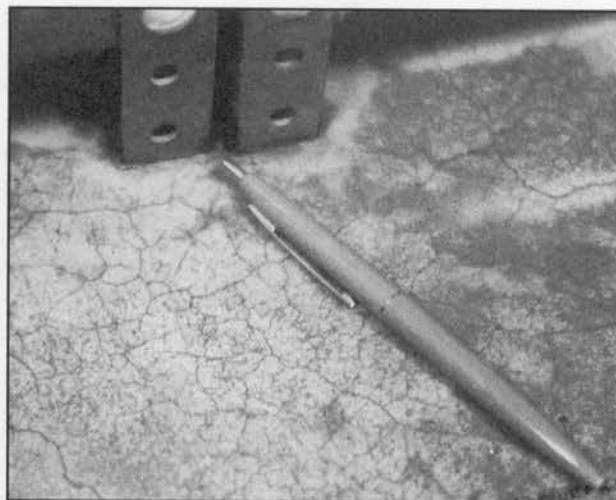
Crazing Concrete Surface (Dampened)
